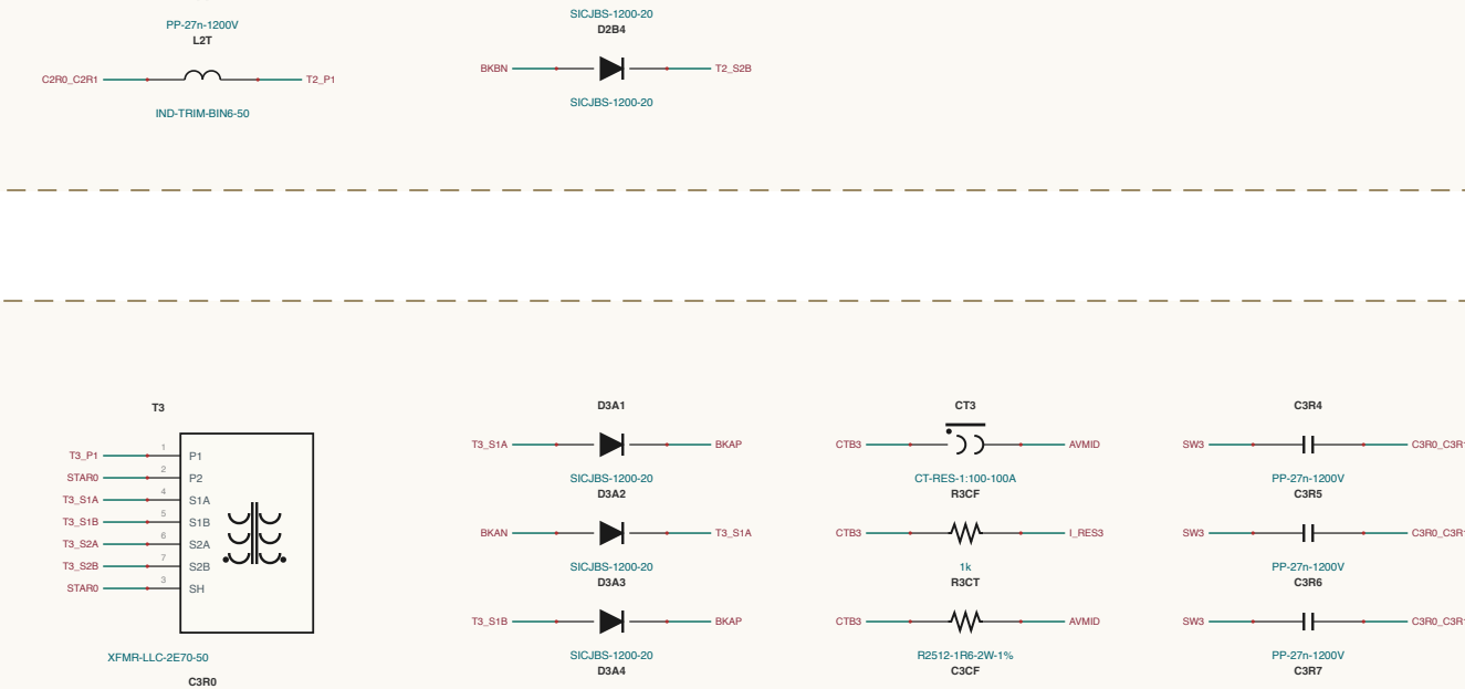
LLC-TANKS / TANK-3
