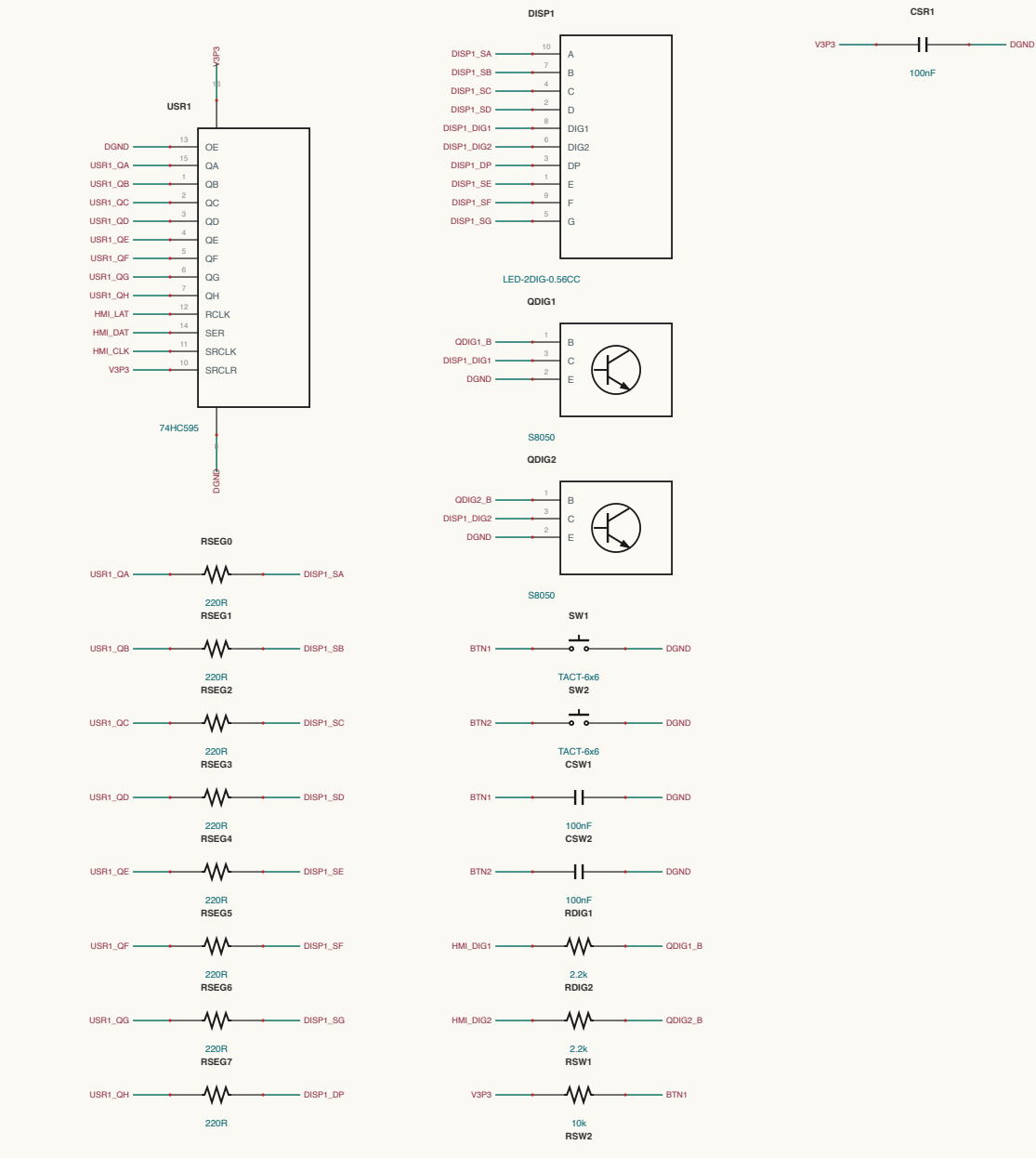
CONTROL / INTERCONNECT
